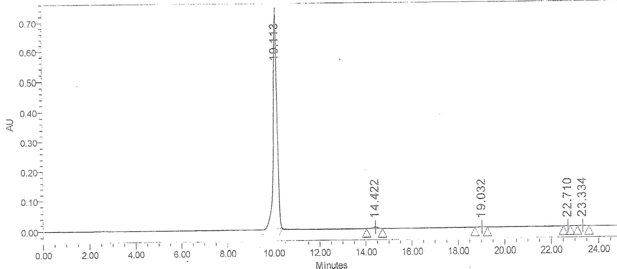
Auto-Scaled Chromatogram
